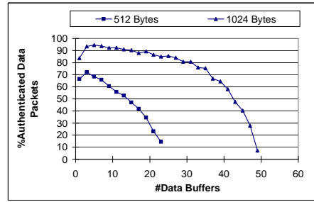
Fig. 7. The performance with different buffer allocation schemes for total memory 512 and 1024 bytes to buffer data and CDM messages. Assume 95% of CDM packets are forged and 50% of packets are lost when transmitted over the channel.
