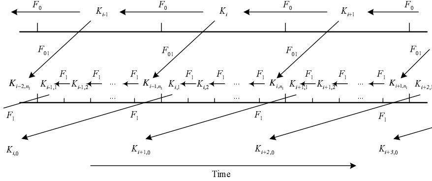
Fig. 3. The two levels of key chains in Scheme III. It differs from Figure 1 in that each K_{i,n_1} is derived from K_{i+1} using an additional pseudo random function F_{01} .
