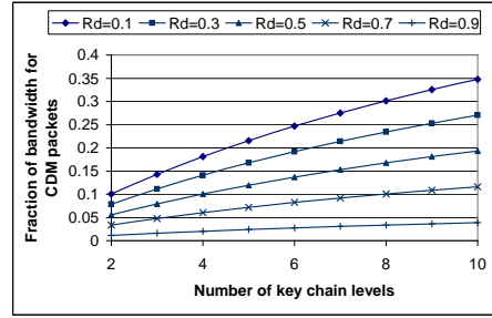
Fig. 6. Bandwidth for CDM messages v.s. number of key chain levels. Assume the number of CDM buffers in each key chain level is m = 40 .
