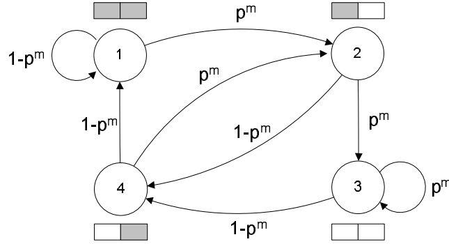
Fig. 4. State transition diagram for Scheme IV
