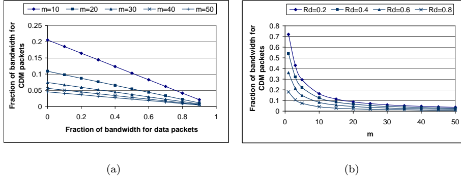
Fig. 5. Bandwidth required for CDM messages to ensure 90% of low-level key chain commitments are authenticated before the key chains are used.
